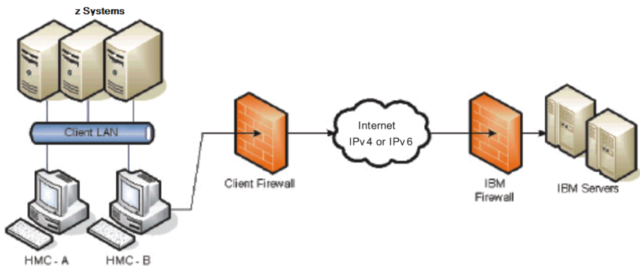
Figure 1. Separating Ethernet adapters
